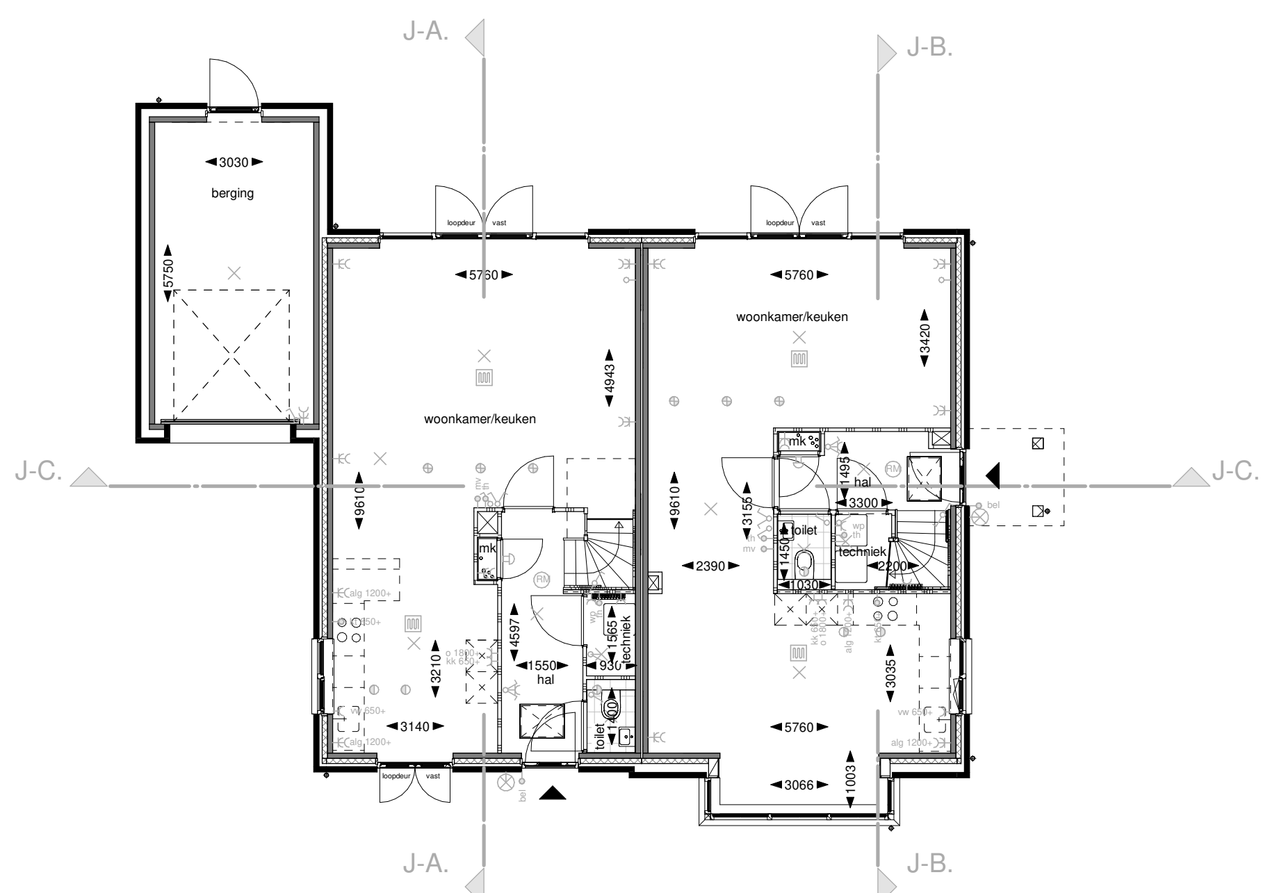
Type: V.60.10 bwnr: 37 Type: Z.60.10.2 bwnr: 36 Begane grond
